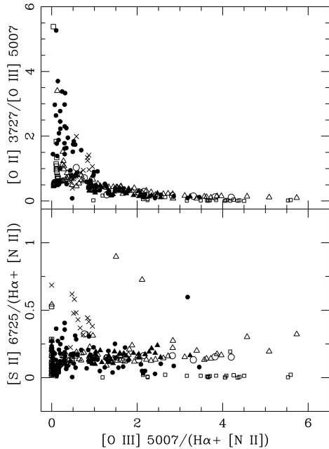
Fig. 2. Diagnostic diagrams for the halo of NGC 6543. Model predictions for HII regions (filled circles, Stasinska (1982)); plane-parallel shock models: Hartigan et al. (1987) (crosses) and Riera (big empty squares, private communication). Small empty squares correspond to observations of type II PNe. Triangles correspond to selected areas of the halo and empty circles correspond to dense structures detected in the halo.
