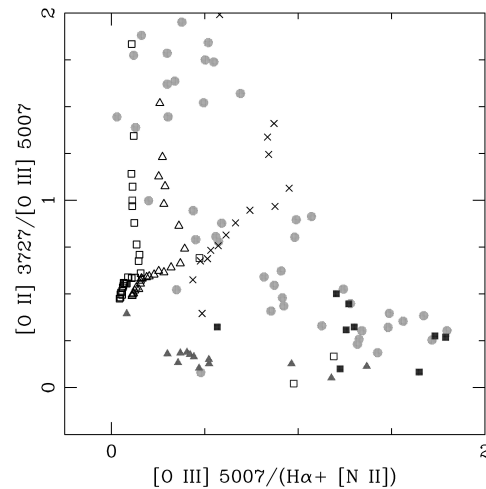
Fig. 1. Diagnostic diagram for NGC 6888. Models predictions for HII regions (circles, Stasinska (1982)); plane-parallel shock models: Hartigan et al. (1987) (crosses) and Riera (empty triangles and empty squares, private communication). Filled squares correspond to observations of type II PNe. Filled triangles correspond to our observations for NGC 6888, obtained in the blown cavity zones.
