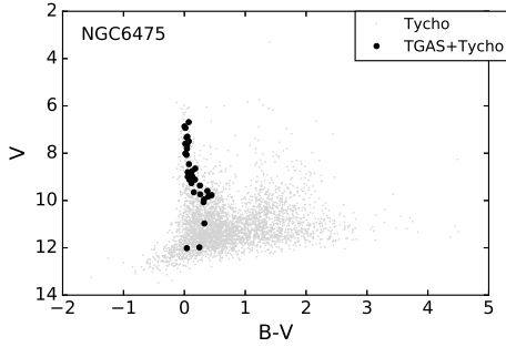
Fig. 1. Colour–magnitude diagram of the cluster NGC6475. The light grey points are the data from Tycho and the black points are the cross-match between the result of the selection from TGAS and Tycho. TGAS data was chosen in a circular area with a radius of 3 degrees around the center.
