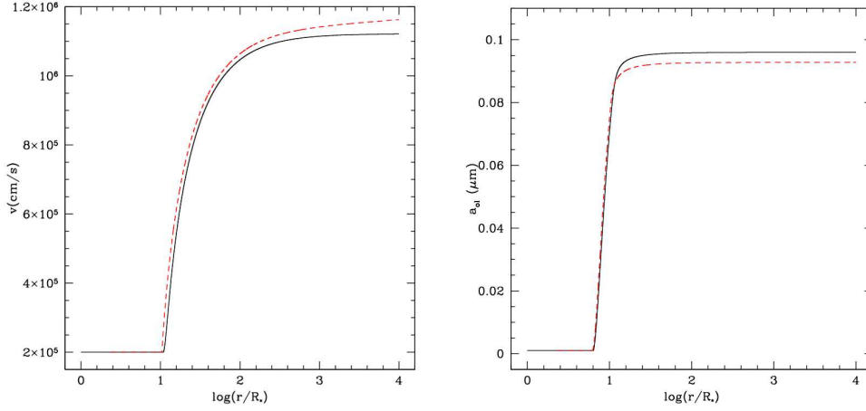
Fig. 1. Left: wind-velocity profiles (note: \text{cm s}^{-1} ) with (red, dashed) gas pressure and without (black, solid). Inside the condensation radius the wind velocity is set to 2 \text{ km s}^{-1} to avoid numerical issues. Right: increase of the grain radius as a function of distance from the centre of the star. The examples shows the case of olivine-type dust.
