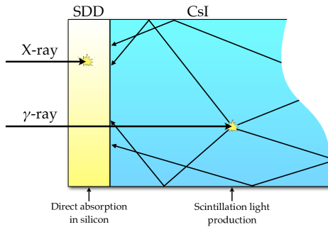
Fig. 1. The siswich architecture.
