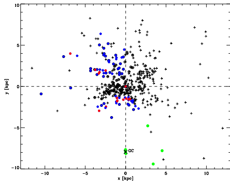
Fig. 1. Distribution of Cepheids on the Galactic Plane. Sun is located at the center of the axis, the black cross indicates the Galactic Center (GC). Our new (red and blue filled circles) optical sample will integrate the metallicity estimates currently available for Cepheids (black crosses: Luck & Lambert 2011; open circles: Pedicelli et al. 2009, 2010; Lemasle et al. 2007, 2008; Romaniello et al. 2008); thanks to new 6 Cepheids (green filled circles) observed in K_s band we will provide new information about the Cepheid metallicity also in the Galactic Bulge and in the GC.
