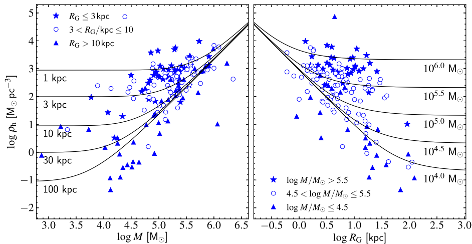
Fig. 1. Isochrones based on the balanced evolution model of Section 2. In the left panel 5 isochrones for different R_G values are shown and in the right panel 5 isochrones for different M . Both panels show the 141 globular clusters in the Harris (1996) catalogue from which M , r_h and R_G are available. In both panels different symbols are used for data in different R_G and M regimes.
