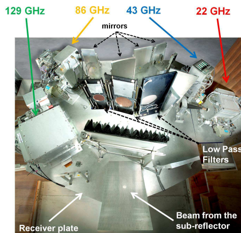
Fig. 1. KVN 4 channel receiving system (Han et al. 2008)
