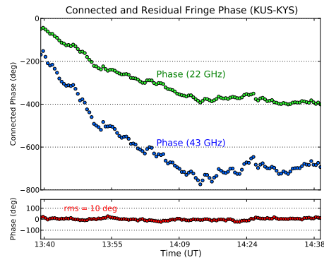
Fig. 3. The fringe phases (22/43 GHz) and residual phase (43 GHz) of the MFPR experiment at the KVN Yonsei-Ulsan baseline
