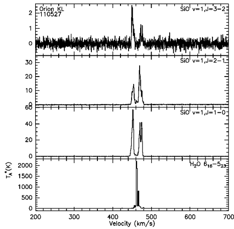
Fig. 2. First simultaneous 22/43/86/129 GHz maser lines from the single dish observation towards Orion KL
