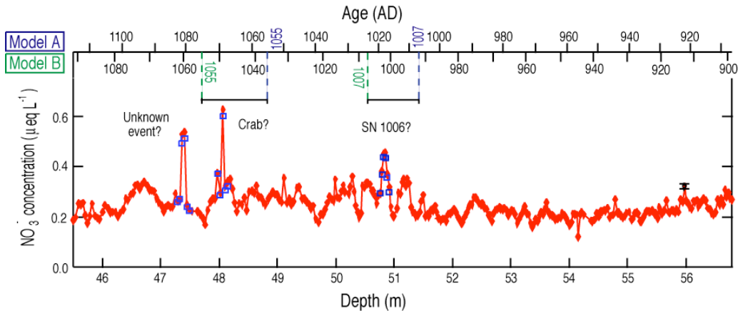
Fig. 1. Nitrate ion spikes in 11th century(from Motizuki et al.2009). There exist three prominent groups of nitrate ion spikes,earlier two are SN1006 and SN1054,but last group consist of two close spikes separated by one year had been unknown.However these "unknown event?" are possible records of R Aquarii in A.D.1073 and A.D.1074 because this group locates between A.D.1060 and A.D.1080.
