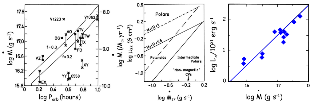
Fig. 1. Left panel: Intermediate polars in the plane \dot{M} - P_{\text{orb}} . The two lines are lines of disc stability: stable above and dwarf nova outburst below. They were computed for f=0.2 and 0.3 , with R_{\text{out}} = f \times a , being a the separation of the two stars in the system (by courtesy of Warner, 1996). Central panel: Magnetic moment in units of 10^{33} G \text{cm}^3 versus mass accretion rate in units of 10^{17} g \text{s}^{-1} . Boundaries for white dwarf mass M_1 = 1 M_{\odot} and M_1 = 0.6 M_{\odot} have been computed for P_{\text{orb}} = 4 h (by courtesy of Warner, 1996). Right panel: Mass transfer rate onto white dwarf versus (2-10 keV) X-ray luminosity (by courtesy of Warner, 1996).
