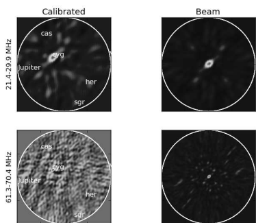
Fig. 1. Top and bottom show respectively the low and high frequency LWA-1 all-sky calibrated image (left) and beam pattern (right) taken using the TBW during commissioning.
