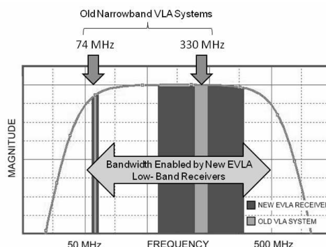
Fig. 2. Available bandwidth for new EVLA broadband low frequency receiver. Old VLA bandwidth shown in light grey and new EVLA bandwidth shown in dark grey. Additional channels exist for future broadband feeds and the curve shows the full available bandwidth.
