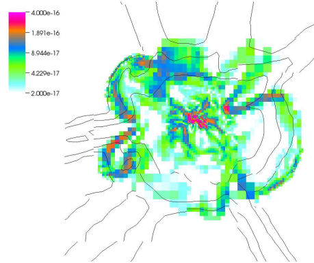
Fig. 2. Slice of 7 \times 7 \text{ Mpc } h^{-1} , showing the vorticity \omega^2 for our reference cluster at z = 0.05 . The vorticity is colour coded, whereas the density is represented as contours, in order to better highlight the filaments surrounding the cluster.
