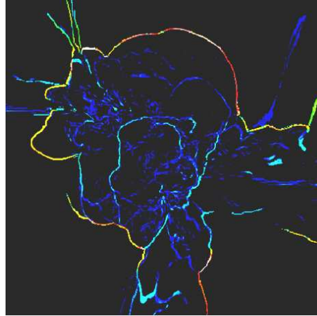
Fig. 2. 2-dimensional slice showing the Mach number of shocks for cluster E1 of our sample. The side of the slice is 13 Mpc/h and the depth along the line of sight is 25 kpc/h.
