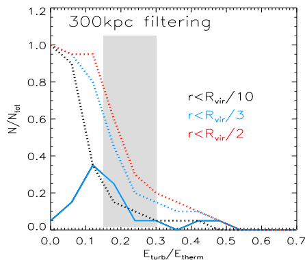
Fig. 6. Cumulative distribution function for E_{\text{turb}}/E_{\text{therm}} inside R_{\text{vir}}/2 , R_{\text{vir}}/3 and R_{\text{vir}}/10 for the simulated clusters assuming l < 300 kpc for turbulence. The solid line shows the differential distributions for R_{\text{vir}}/3 . The grey band shows the turbulence required in the turbulent re-acceleration scenario (e.g. Brunetti & Lazarian 2010).
