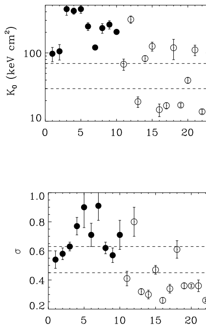
Figure 1. Cool core indicators ( K_0 and \sigma ) for all the clusters in the sample. Filled symbols are “radio-loud” clusters while open symbols are radio-quiet.
