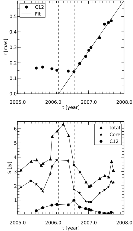
Fig. 2. Top panel: Evolution of the separation from the VLBI core of component C12. Bottom panel: Flux density evolution of component C12, the VLBI core and the total flux density. The uncertainties in the flux densities are around 5% and the positional errors are \sim 1/5 of the restoring beam size (typically around 0.1 mas)
