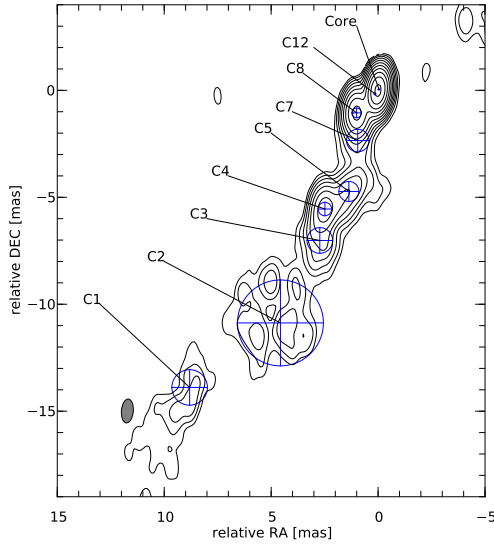
Fig. 1. 15 GHz VLBI image of CTA 102 with fitted circular Gaussian components observed on 6th of January 2007. The map peak flux is 1.13 Jy/beam, where the convolving beam is 1.1 \times 0.6 mas at P. A. -4.8^\circ .
