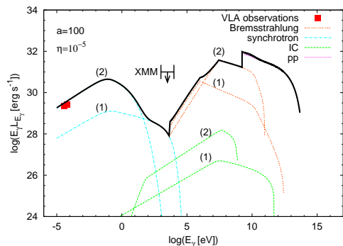
Fig. 1. Spectral energy distribution of the termination point of the jet of a massive young stellar object (Araudo et al. 2007).
