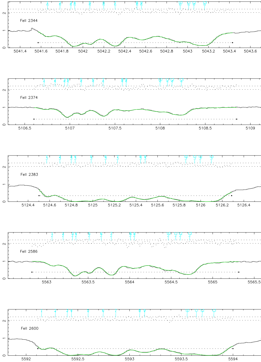
Fig. 1. The 5 Fe II lines of the z_{\text{abs}}=1.15 in HE 0515 – 4414 are shown. The fit is obtained with VPFIT by using 13 components ( \chi^2=1.1 ). Treating the Fe II \lambda\lambda 2383 as Mg II \lambda\lambda 2804 the whole set of lines would provide a spurious signal at \delta\alpha/\alpha = (-11.9 \pm 2.5) \cdot 10^{-6} .
