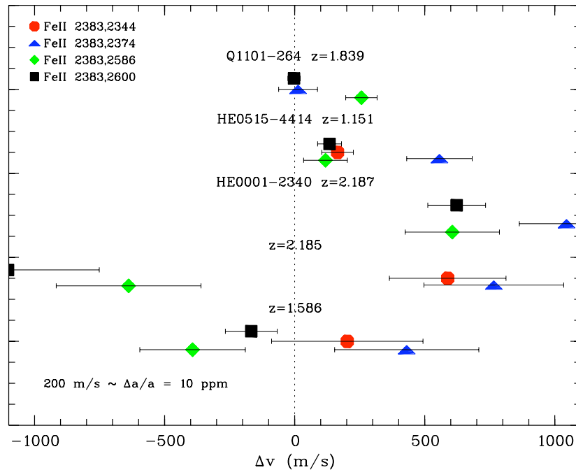
Fig. 2. Velocity shifts between the 5 Fe II lines which share almost identical sensitivity to changes in the fine structure constant (ppm, part per million = 10^{-6} ).
