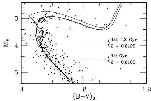
Fig. 2. Comparison of isochrones for the indicated ages and metallicities with the Montgomery et al. (1993) CMD of M 67, assuming E(B - V) = 0.038 and (m - M)_V = 9.70 . The vertical line bounded by short horizontal lines, located just to the left of the turnoff, indicates our estimate of the gap location. Only the dashed isochrone has a blueward hook in the same magnitude range. The 3.6 Gyr isochrone for Z = 0.0125 has a very similar morphology to the dashed isochrone, but the predicted location of the gap (the blueward hook) is significantly too bright if best estimates of the reddening and distance are assumed.
