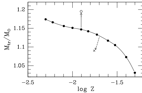
Fig. 1. The filled circles, connected by a solid curve, give the dependence on Z of the mass of the lowest mass star that is predicted to have a convective core at the end of the MS phase: at a given Z , masses below the solid curve have radiative cores. [These results, which are reproduced from VandenBerg et al. (2006), assume Z_{\odot} = 0.0188 and the distribution of heavy element abundances reported by Grevesse & Noels (1993).] The open circle indicates the value of \mathcal{M}_{\text{tr}} if Z_{\odot} = 0.0125 , assuming the Asplund et al. (2006) metals mixture, whereas the cross indicates the expected effect of diffusive processes on \mathcal{M}_{\text{tr}} , based on the computations by Michaud et al. (2004). As indicated by the dashed line, diffusive models predict that the metallicity in the surface layers of the Sun will decrease to \approx 0.0175 at the solar age if Z \approx 0.02 initially.
