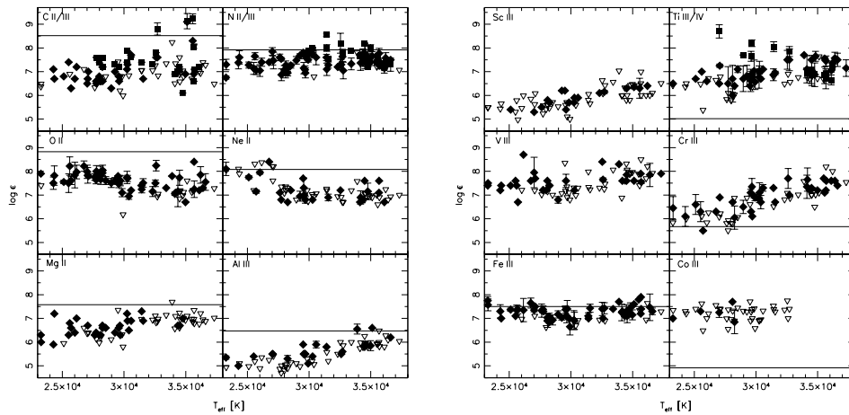
Fig. 1. The abundances of selected elements are plotted against the effective temperature. If two ionization stages are present, the lower one is marked by diamonds, the higher one by rectangles. Open triangles mark upper limits. Solar abundances (Grevesse & Sauval 1998) are drawn as horizontal lines. The solar abundances of scandium ( \log \epsilon_{\text{Sc}} = 3.17 ) and vanadium ( \log \epsilon_{\text{V}} = 4.00 ) are below the plotted range.
