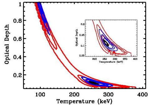
Fig. 4. Contour plots \tau-kT_e for simulations of different exposures (red: 1ks, blue: 5 ks and black: 50 ks). The simulated data correspond to a thermal comptonization spectrum with L_{2-10keV} = 10^{-11} erg.s-1.cm-2, kT_e = 250 keV, \tau = 0 . Only the long exposure simulation enable to break the \tau-kT_e degeneracy characteristic of thermal comptonization spectra.
