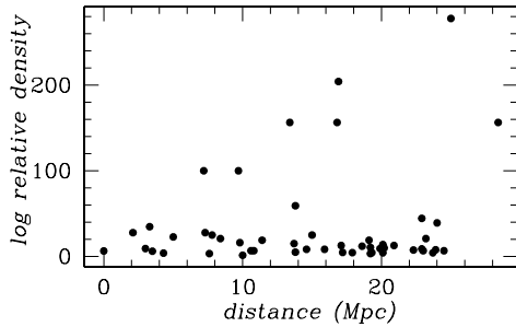
Fig. 1. The dependence of group density with distance from a sample of 50 galaxy groups taken from Tully (1987). Most groups are much like the Local Group in their average density.
