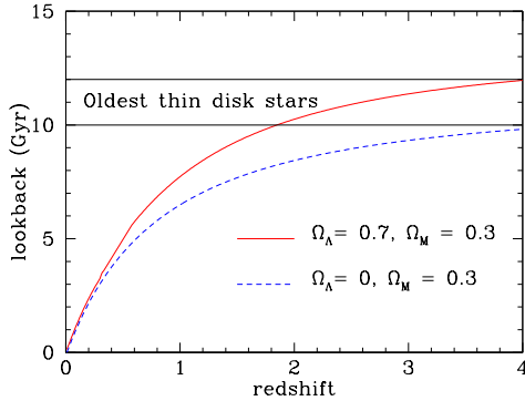
Fig. 1. Plot of lookback time versus redshift for two cosmological models, as labelled, each with present value of the Hubble constant of 70 km/s/Mpc. The horizontal lines indicate estimates of the ages of the oldest stars in the thin disk, from Binney et al. (2000).
