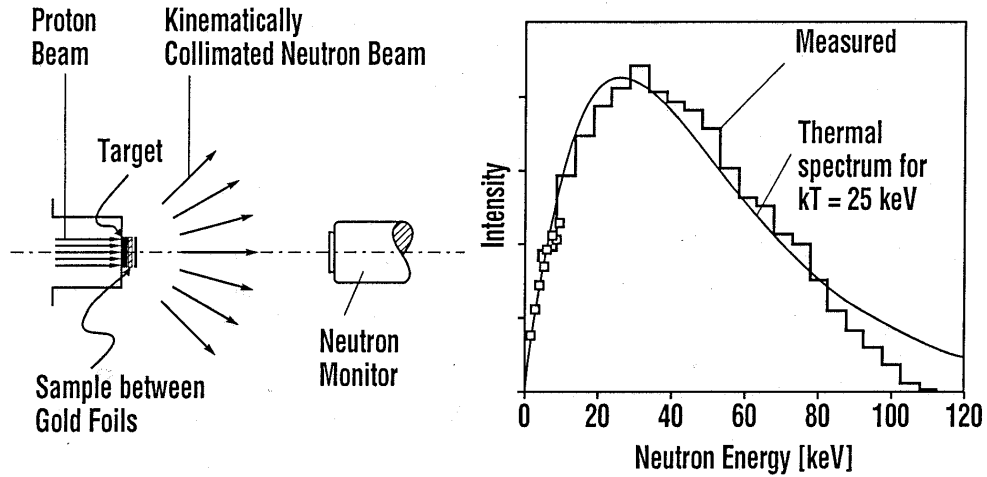
Fig. 2. The experimental setup for activation measurements (left), and a comparison of the produced neutron spectrum and a thermal neutron spectrum at kT=25 keV (right).
