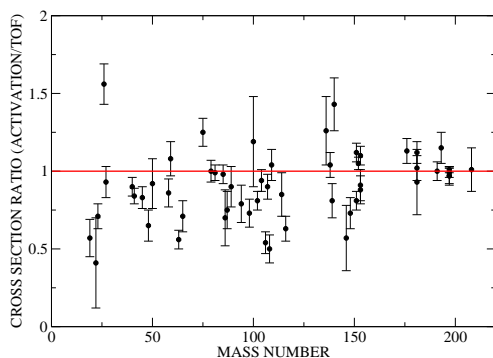
Fig. 3. Comparison of MACSs at kT=30 keV obtained by the activation and TOF method.
