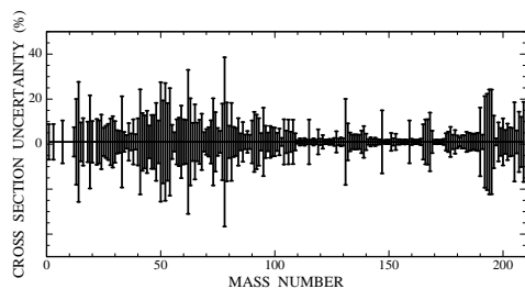
Fig. 1. Uncertainties of Maxwellian averaged neutron capture cross sections at a thermal energy of kT=30 keV.
