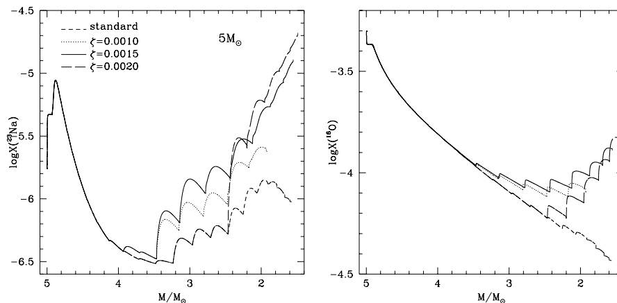
Fig. 1. Variation with mass of the surface abundance of Sodium (left), and Oxygen (right) during the AGB evolution of a model with initial mass M = 5M_{\odot} calculated with various values of the extra-mixing parameter \zeta .
