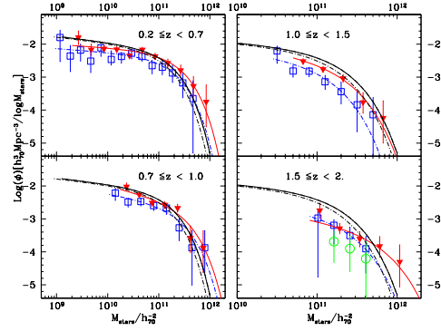
Fig. 5. Stellar mass functions in the K20 sample. Different symbols correspond to different methods adopted to estimate the stellar mass Fontana et al. (2004). In the highest redshift bin, large hollow circles correspond to objects with only spectroscopic redshift. The thick solid line is the local galaxy mass function (?).
