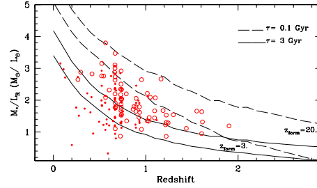
Fig. 3. M_{stars}/L_R ratio as a function of redshift for the spectroscopically identified ETGs in the the K20 sample. Large hollow and small filled circles indicate M_R < -22 and M_R > -22 respectively. Lines show M_{stars}/L_R values predicted for a set of exponentially-decaying star formation rate models with z_f = 3 (thin lines) or z_f = 20 (thick lines) and time-scales of \tau = 0.1 Gyr (dashed lines) and \tau = 3 Gyr (solid lines) (Salpeter IMF and no dust extinction) Fontana et al. (2004).
