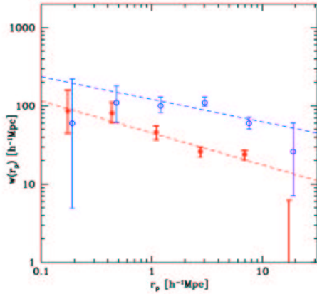
Fig. 9. Projected correlation functions of X-ray sources in the CDFS (open circles) and CDFN (filled circles, Gilli et al. 2005).
