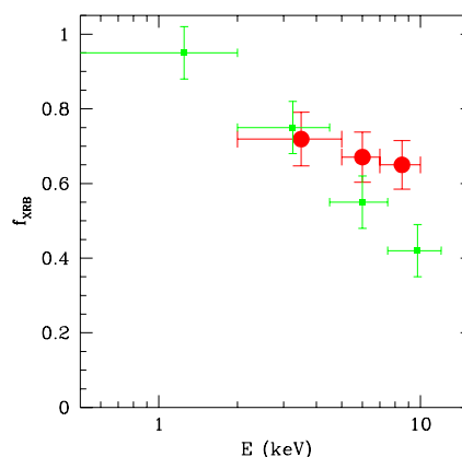
Fig. 4. Red circles: contribution to the resolved XRB in the CDFS in different energy bands. Small green squares are from Worsley et al. (2005).
