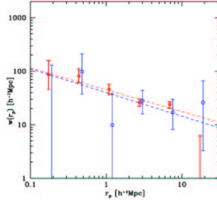
Fig. 10. Spatial correlation functions in the CDFS (open circles) after removal of the two major spikes compared with that measured in the CDFN (filled circles, Gilli et al. 2005).
