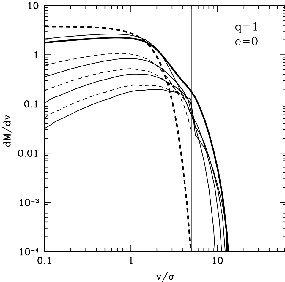
Fig. 1. Stellar velocity distribution (normalized to the total mass of interacting stars in units of the total binary mass M ) for an equal mass, circular binary, at different stages of the hardening. The vertical line marks v_{\text{esc}} \simeq 5\sigma . Dashed lines : from top to bottom, distribution of stars in the shrinking loss cone before the 1st, 2nd, 3rd and 4th iteration. For clarity, the initial loss cone distribution is marked with a thicker line. Thin solid lines : from top to bottom, distribution of stars which have received 1, 2, 3 and 4 kicks. Thick solid line : final stellar velocity distribution after loss cone depletion is completed.
