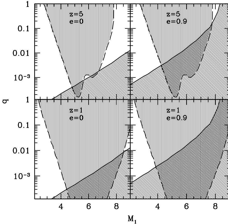
Fig. 4. In the plane M_1 - q , the vertical shaded area limits LISA potential targets with SNR > 5 . The diagonal shaded area on the lower right corner marks binaries that are going to coalesce within 5 Gyrs after loss cone depletion. In each panel, the reference redshift and eccentricity of the MBHBs are labelled.
