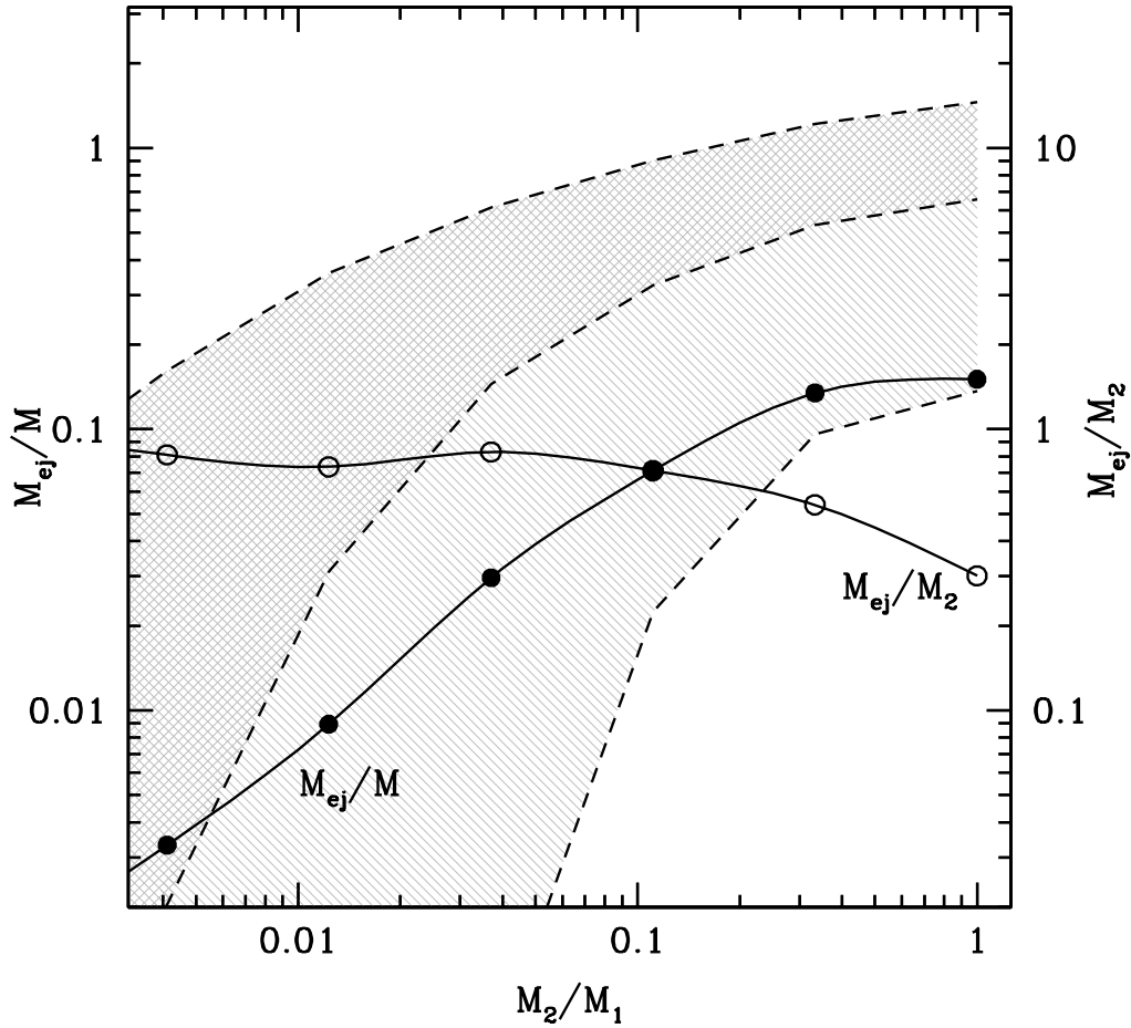
Fig. 3. Ejected stellar mass M_{ej} normalized to the total binary mass M (left scale, solid points), and to the mass of the lighter binary member M_2 (right scale, empty points), as a function of the binary mass ratio. The curves are polynomial interpolations. Note that M_{ej}/M and M_{ej}/M_2 does not depend on the absolute value of M , and are nearly independent on e . The upper, dark shaded area defines the mass (normalized to M ) a M = 10^6 M_\odot binary needs to eject to reach a final separation a_f such that t_{GW} = 1 Gyr. Upper and lower limits to the area are for e = 0 and e = 0.9 , respectively. The lower, light shaded area is analogous, but for a M = 10^9 M_\odot binary. Incidentally, the e = 0.9 limit for the light binary practically coincides with the e = 0 limit of the heavy one.
