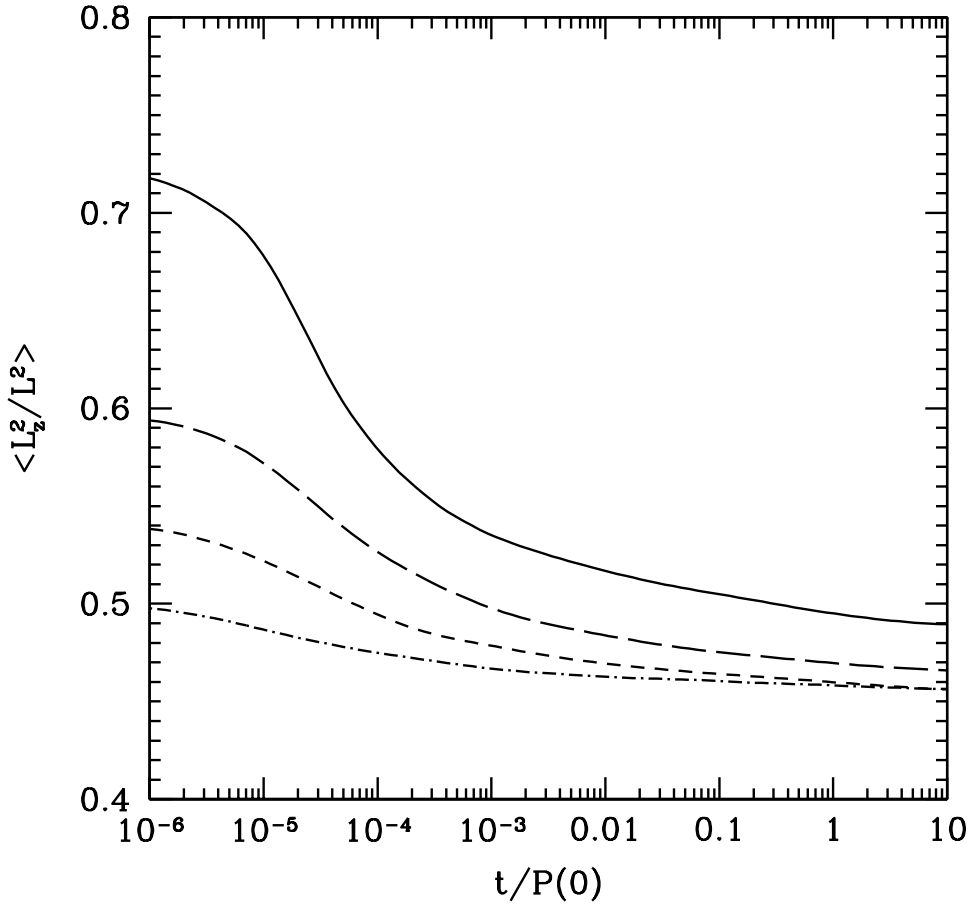
Fig. 2. Time evolution of angular momentum of ejected stars, in terms of L_{z\star}^2/L_\star^2 , for a circular binary, and, from bottom to top, for q=1/27, 1/9, 1/3 and 1
