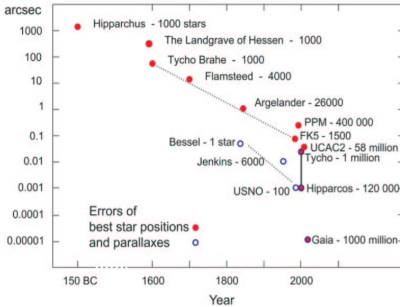
Fig. 1. Astrometric precision throughout of history (from E.Hoeg).
