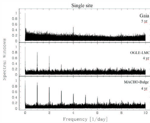
Fig. 3. Spectral window of Gaia (top), and two other surveys OGLE (middle), MACHO (bottom). The spectral windows of single site makes them prone to high peaks, which when convolved with the signal will produce aliasing frequencies. The visibility of the bulge makes the spectral window particularly prone to high peaks.
