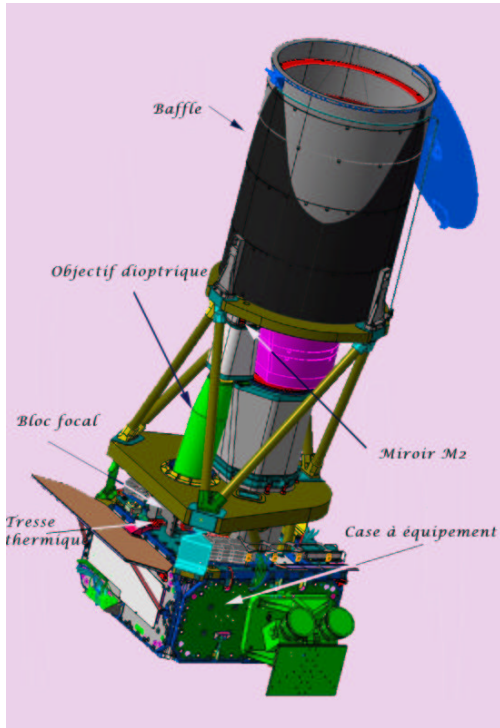
Fig. 1. Schematic representation of CoRoT.
