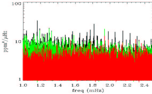
Fig. 6. Same as Fig.4 for HD49385.
