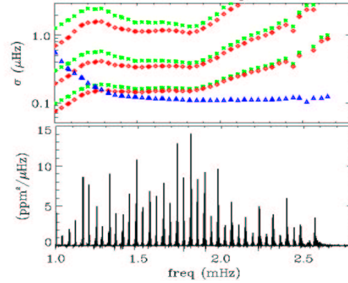
Fig. 7. same as Fig.5, for HD49385.
