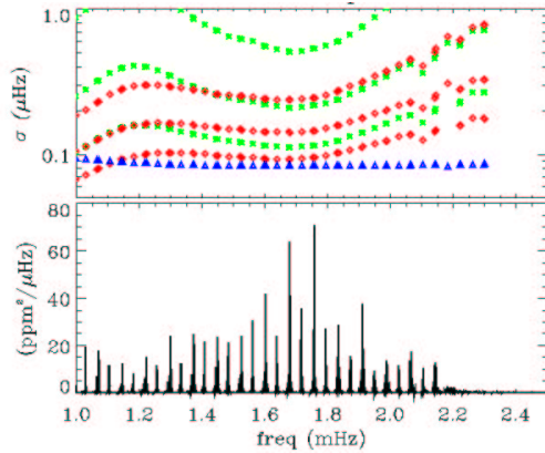
Fig. 5. Lower panel: simulation of the pure seismic signal expected for HD49933. Upper panel: Estimates of the 1\text{-}\sigma precision on the determination of eigenfrequencies, for case a, b and c (resp. triangles, rhombs, stars) as described in the text.
