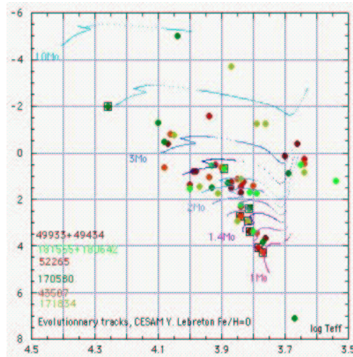
Fig. 8. The CoRoT HR diagramme. Illustration of what could be the set of objects observed during 150d runs after 3 years.
