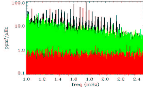
Fig. 4. Simulation of the power spectrum expected for HD49933, including photon noise (dark grey) and granulation noise (light grey) estimates as described in the text.
