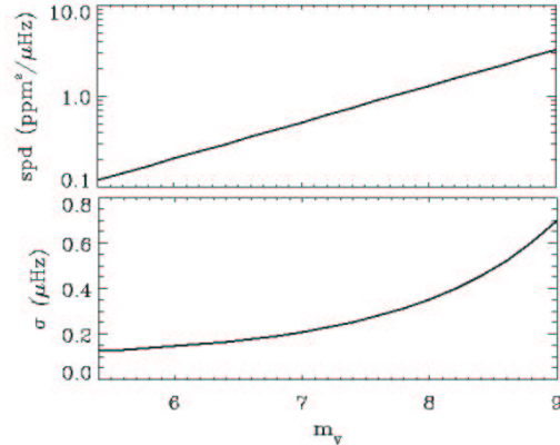
Fig. 3. Upper panel: Photometric performance expected for CoRoT (spectral power density) for the range of m_V considered. Lower panel: 1-\sigma precision estimate for mode amplitudes and lifetimes taken from the Sun.
