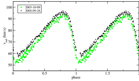
Fig. 1. RV curve of RS Gru phased with P=0.147d .
