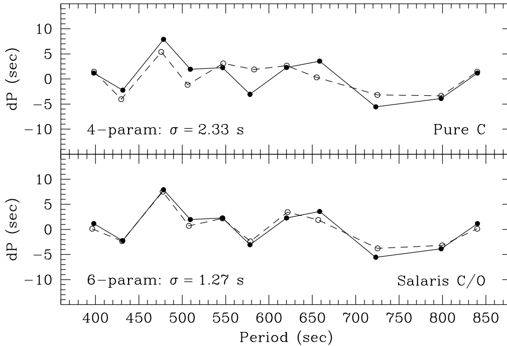
Fig. 1. A comparison of the optimal match (open points) to the observed periods of CBS 114 (solid points) for double-layered envelope models with a pure C core (top panel) and an adjustable C/O core motivated by the calculations of Salaris et al. (1997, bottom panel). The addition of two free parameters is expected to improve the fit from \sigma_p = 2.33 s to 1.87 s, but the fit actually improves by more than twice this amount.
