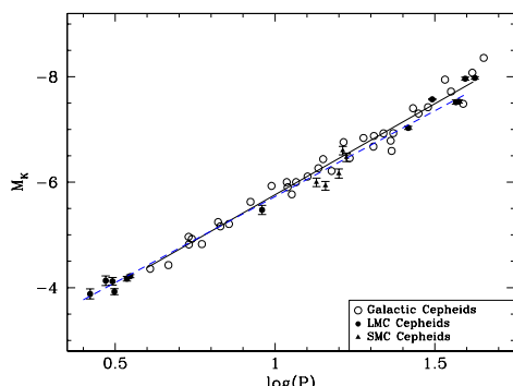
Fig. 4. Absolute ISB-based K-band PL relations in Milky Way and LMC, calculated from the revised p-factor law. Solid line is the best fit to the Milky Way data. This line fits also the LMC data very well. The dashed line is the Persson et al. PL relation for LMC Cepheids, which now agrees very well with the ISB-based Milky Way and LMC PL relations.
