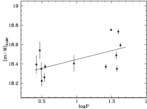
Fig. 2. ISB-determined true distance moduli for LMC Cepheids, calculated with the canonical p-factor law. The distance moduli have been corrected for the tilt of the LMC plane with respect to the line of sight. There is a significant trend of the distance moduli with period.
