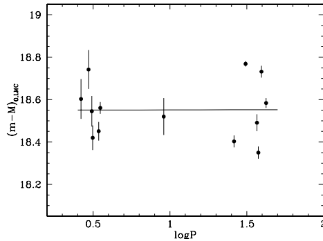
Fig. 3. As Fig. 2, but now distance moduli calculated with the revised p-factor law of this paper. The trend in Fig. 2 has disappeared.
