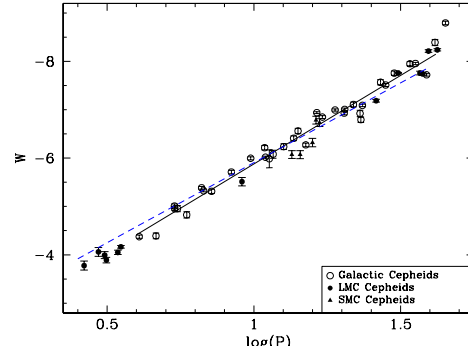
Fig. 1. Absolute W-band magnitudes derived from the ISB distances of 38 Milky Way, 13 LMC and 5 SMC Cepheids. The canonical p-factor relation was used for the ISB distance calculation for all stars. The solid line is the best fit to the Milky Way data. The dashed line is the W-band PL relation in the LMC from the OGLE-II project, for an assumed LMC distance modulus of 18.50. The ISB-based PL relations both in Milky Way and LMC are significantly steeper than the OGLE-II LMC relation.
