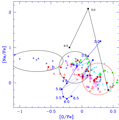
Fig. 1. : O-Na anti-correlation for the stars of several globular clusters. NGC 2808 is labelled by full dots (Carretta et al. 2004). The models by Ventura & D’Antona (2005) are labelled by masses from 3 to 6.5 M_{\odot} , the models by Fenner et al. (2004) by dots of 3.5, 5 and 6.5 M_{\odot} . The circle at the right includes the ‘normal’ stars (first generation); the models should explain the abundances in the intermediate circle. The left circle stars, the most extreme, remain unexplained till now.
