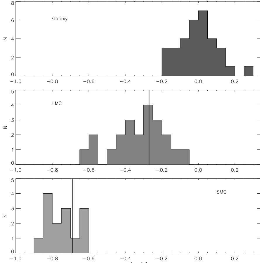
Fig. 1. Histograms of the [\text{Fe}/\text{H}] ratios derived for all the stars of our sample in the Galaxy, the LMC and the SMC. The solid lines indicate the mean values found using F and K supergiants by Hill et al. (1995) and Hill (1997).
