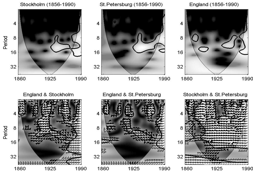
Fig. 3. Wavelet transforms of the standardized time series. The 5% significance level against red noise is shown as a thick contour. Cross-wavelet spectra are displayed at the bottom of the panel. The relative phase relationship is shown as arrows (with in-phase pointing right, anti-phase pointing left, and one set of data leading another by 90 pointing straight down).
