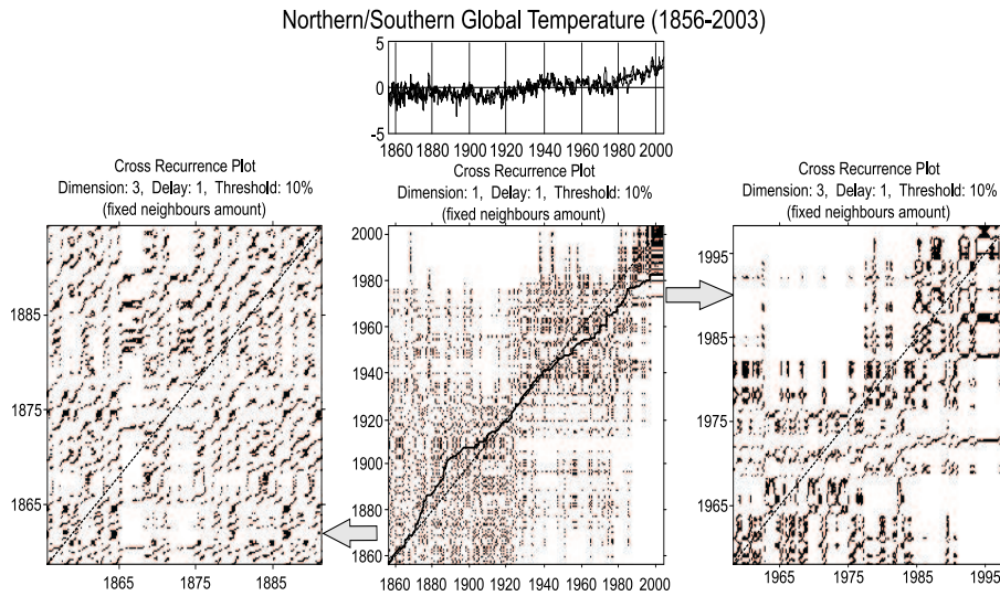
Fig. 4. Cross Recurrence Plots demonstrate synchronous changes in the monthly mean temperatures of the Northern and Southern Hemispheres. However, the density of plots is asymmetrical denoting a slight bowing of the line of synchronization (solid line) relative to the main diagonal (dashed line). The texture of CRP is significantly different in the late of last decades of 19th and 20th centuries.
