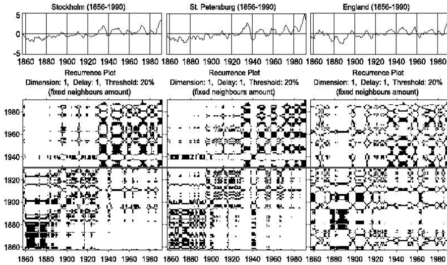
Fig. 2. Recurrence plots of the air surface temperature in Stockholm, St.Petersburg and Central England versus time from 1856 to 1990. Note the near-simultaneous phase transitions observed in late of 1930's. Patterns just before and after this time are different denoting different recurrent behavior of underlying dynamical systems. The demarcation line corresponding to structural changes is marked by horizontal line.
