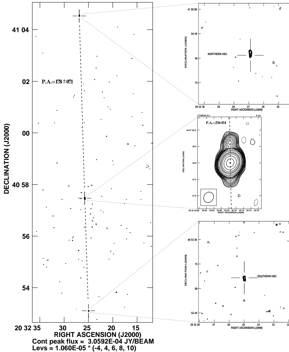
Fig. 1. Natural weight 6 cm map of the Cygnus X-3 field. This map covers almost the totality of the antenna primary beam and shows the existence of two radio sources perfectly aligned with the PA of the inner radio jets. A close-up look at the locations is given on the right top and bottom panels. Note the remarkable effect of the bandwidth smearing that affected the archival data which caused the sources to appear elongated. The central panel was taken from Marti et al 2001 and included for illustrative purposes corresponding to other observation of the Cygnus X-3 arc-second radio jets.
