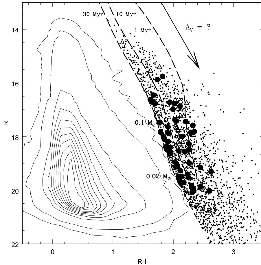
Fig. 1. R, (R - I) color-magnitude diagram for the Upper Sco survey data. Contours indicate the density of sources detected in both R - and I -bands ( \sim 1 million with good photometry in both bands). Data are represented at the 90%, 80%, 70%, 60%, 50%, 40%, 30%, 20%, 10%, 1% and 0.5% levels. Objects which appear younger than 30 Myr based on their location on the color-magnitude diagram are shown as discrete points. Stars identified as variables are drawn as large circles. Spectroscopically observed Upper Sco members from Ardila et al. (2000) are shown as open triangles. We expect low mass cluster members to exhibit only moderate extinction ( A_V < 1 ; Martín et al. 2004).
