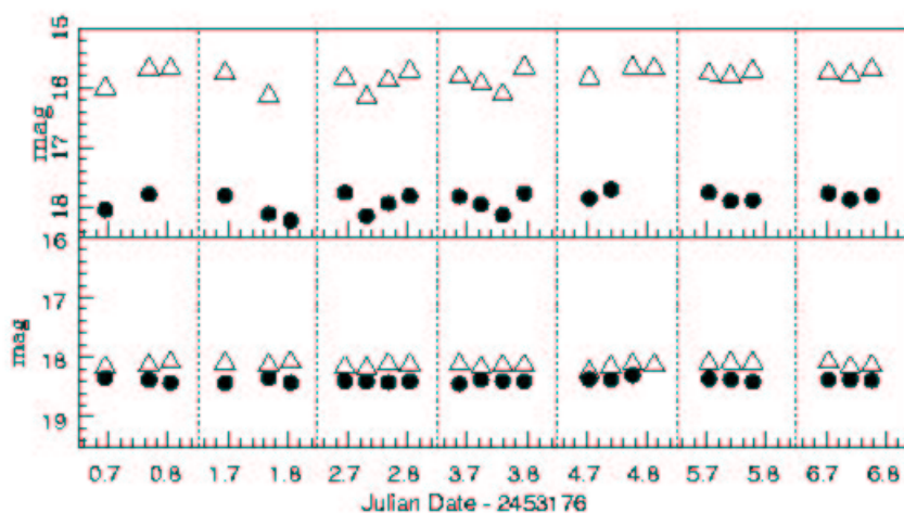
Fig. 2. Upper panels show the light curve of a known low mass pre-main sequence star in Upper Sco (UScoCTIO 100; Ardila et al. 2000) which we found to be variable in our Quest-2 data. Lower panels are the light curve for a nearby ( <20 arcsec) object, shown to demonstrate the quality of the photometry. In all panels open triangles are I -band data and circles are R -band data. Dotted lines represent gaps between nights in the time series.
