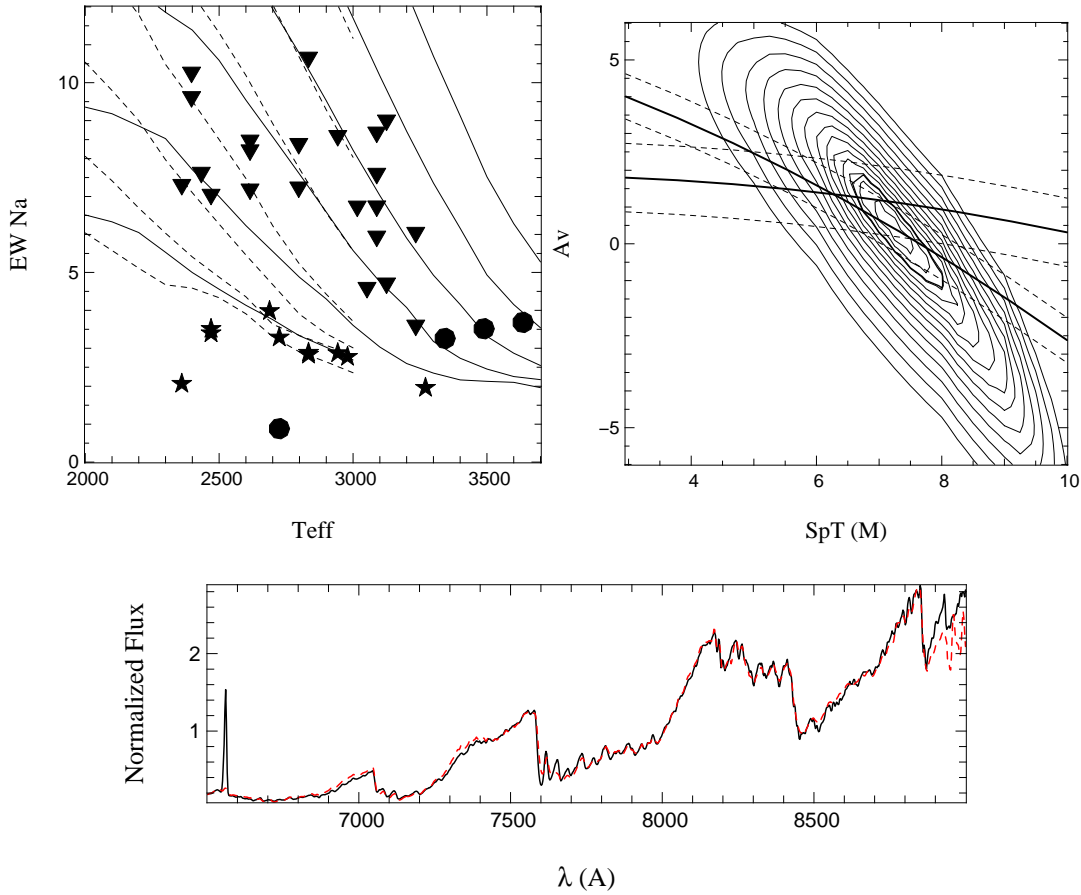
Fig. 1. Top Left: Sodium equivalent width vs effective temperature for our candidate sample. Star symbols represent spectra best fitted with a giant +field-dwarf average (Luminosity class IV). Curves show predictions from the models of Chabrier et al (2000), (solid lines = DUSTY models, dashed lines = COND models) spanning \log_{10}(g/g_{\odot}) = 2.5 to 6.5. Top Right: \chi^2 map obtained in the A_V -SpT plane for one of our candidate spectrum. Also plotted (solid lines) are the A_V variation vs SpT derived from the (I-J) and (J-H) colors using the Rieke & Lebofsky (1985) extinction law. Dashed lines correspond to 1\sigma uncertainties of this calculation. In this example, both our numerical fitting procedure and the colors agree to give an M7.25 Spectral Type and A_V = 0.4 mag. Bottom: The best fit spectrum is shown.
