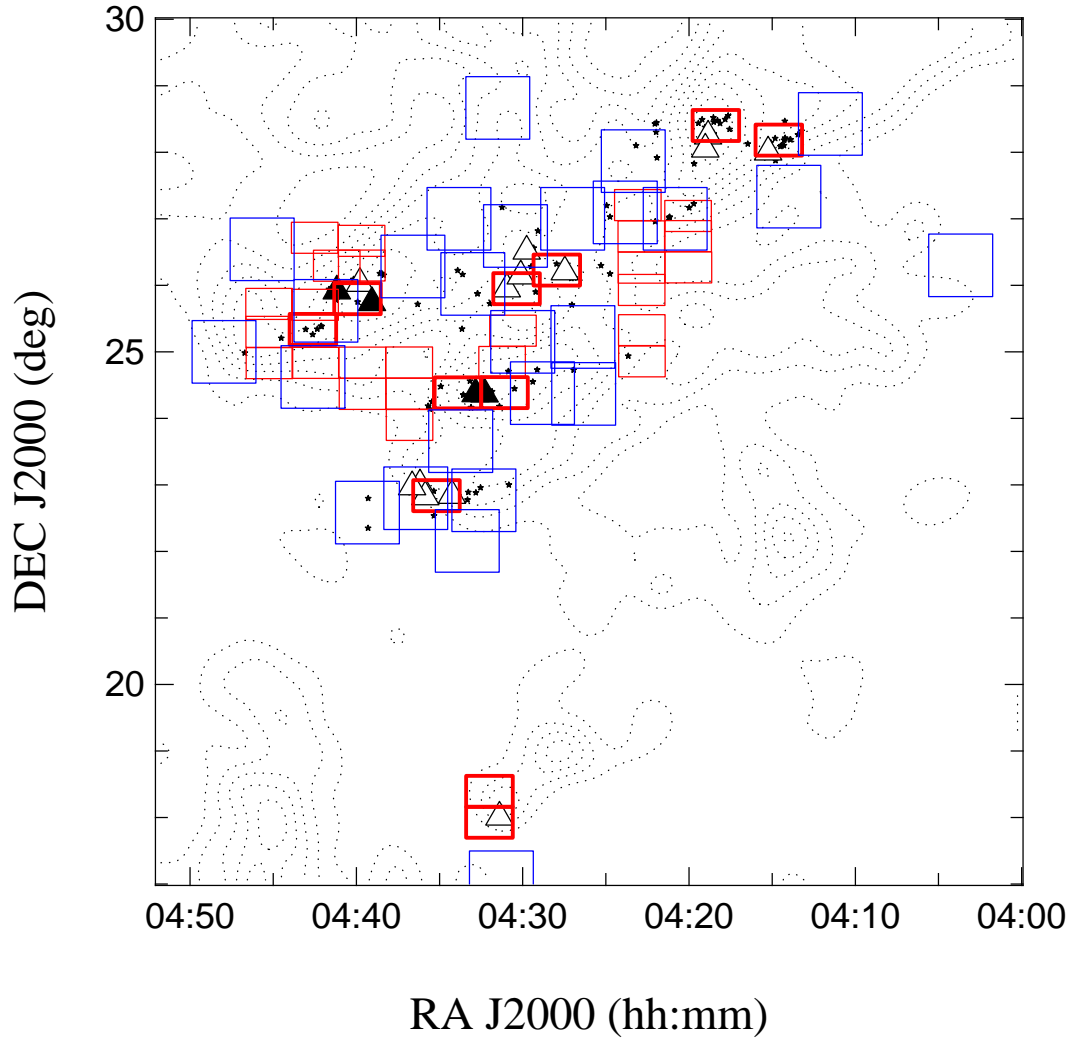
Fig. 2. Total optical survey coverage: red rectangular boxes are CFHT12k fields, and blue square boxes are Megacam fields. Also plotted are known T Tauri stars (star symbol) and known Taurus Brown Dwarfs (triangle), the filled triangles are the 4 Brown Dwarfs discovered in the first CFHT12k 3.6\text{deg}^2 survey (plotted with thick red boxes).
