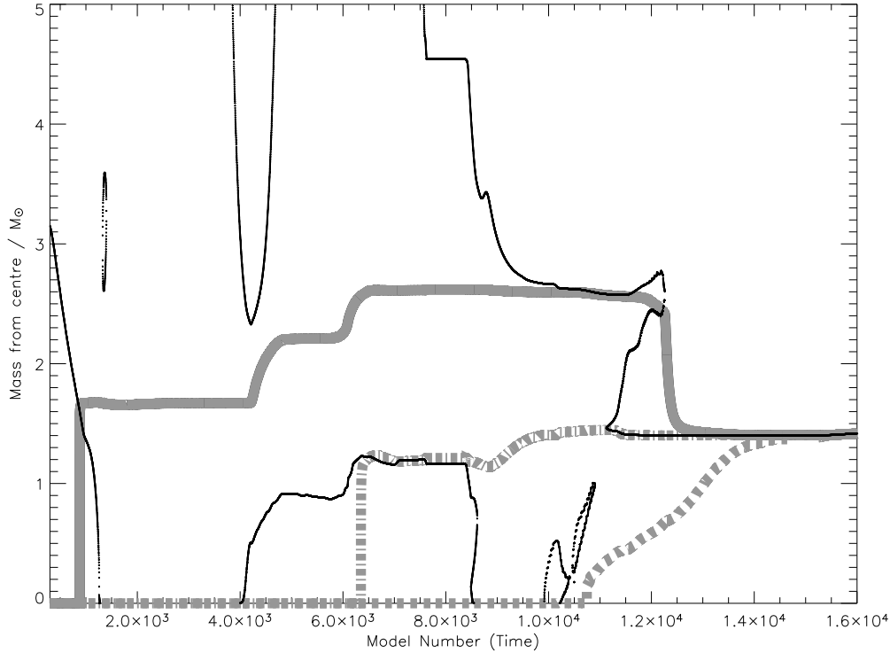
Fig. 1. Evolution of the structure of a 10 M_{\odot} star. The thin black lines show the convective regions while the thick grey lines represent the burning shells. The solid grey line is the hydrogen-burning shell, the dash-dotted line the helium-burning shell and the dashed line the carbon-burning shell. Notice the formation of the convection zone between the hydrogen and helium burning shell at around model 11,000 that reduces the mass of the CO core before second dredge-up.
