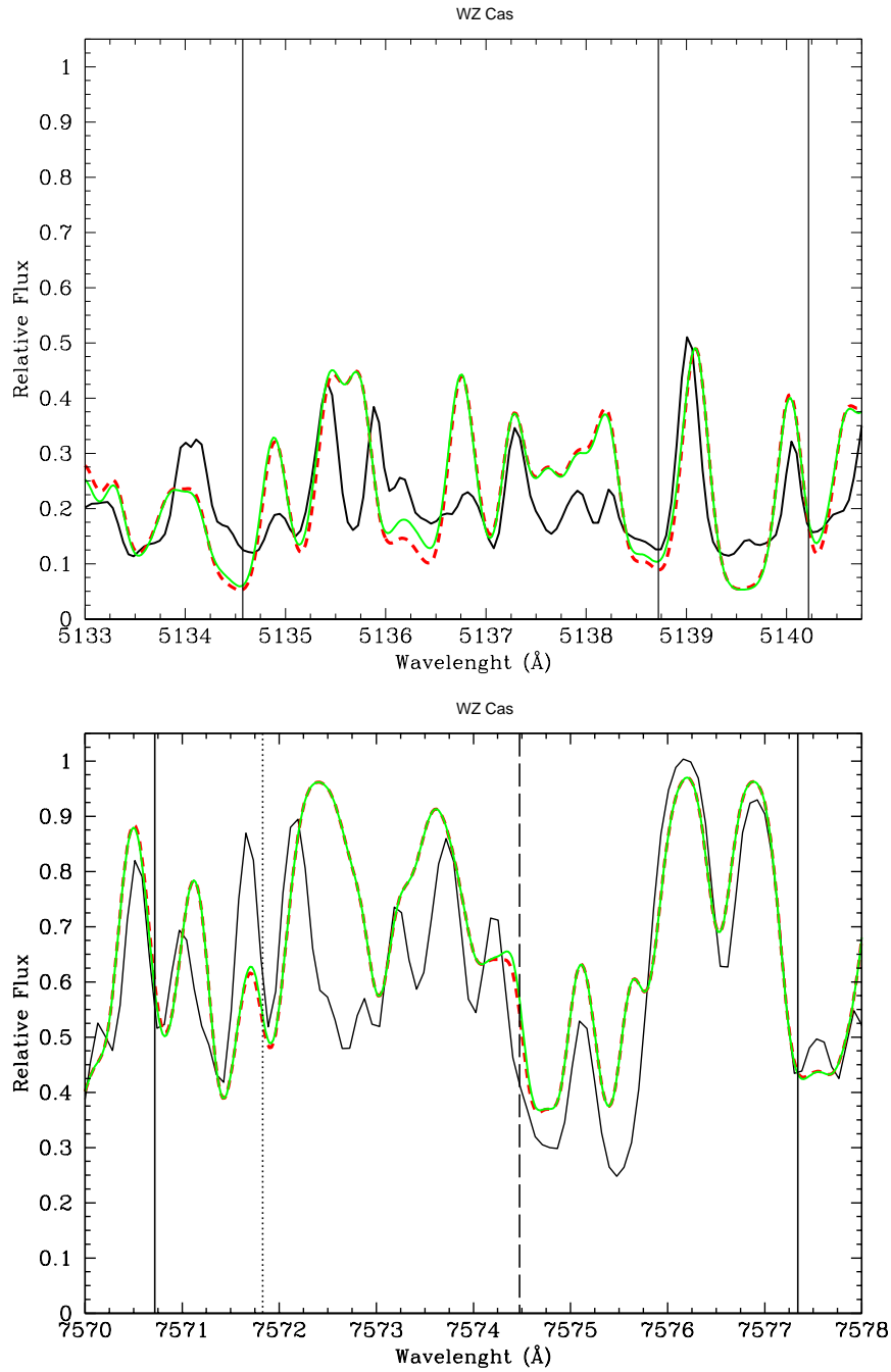
Fig. 2. Spectrum of WZ Cas (thin continuous line). Upper panel: range of 5133 – 5141 Å. The dashed line represents a synthetic spectrum with ^{25}\text{Mg}/^{24}\text{Mg} = 0.13 and ^{26}\text{Mg}/^{24}\text{Mg} = 0.14 (terrestrial Mg ratios); the thick solid line represents a synthetic spectrum with ^{25}\text{Mg}/^{24}\text{Mg} = 0.02 and ^{26}\text{Mg}/^{24}\text{Mg} = 0.06 . Vertical lines have the same meaning as in Figure 1. Lower panel: 7570 – 7578 Å range. The dashed line represents terrestrial isotopic Mg ratios; the thick solid line represents a synthetic spectrum with ^{25}\text{Mg}/^{24}\text{Mg} = 0.02 and ^{26}\text{Mg}/^{24}\text{Mg} = 0.06 . Vertical lines indicate the position of ^{24}\text{MgH} (solid), ^{25}\text{MgH} (dashed) and ^{26}\text{MgH} (dotted) lines.
