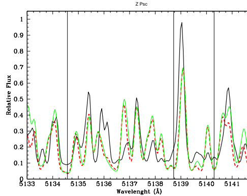
Fig. 1. Spectrum of Z Psc (thin continuous line) in the range 5133 – 5141 Å. The dashed line represents a synthetic spectrum with ^{25}\text{Mg}/^{24}\text{Mg} = 0.13 and ^{26}\text{Mg}/^{24}\text{Mg} = 0.14 (terrestrial ratios); the thick solid line represents a synthetic spectrum with ^{25}\text{Mg}/^{24}\text{Mg} = 0.43 and ^{26}\text{Mg}/^{24}\text{Mg} = 0.44 . Vertical lines indicate the position of ^{24}\text{MgH} transitions. ^{25,26}\text{MgH} lines are located to the left of ^{24}\text{MgH} ones and are not resolved in our spectra.
