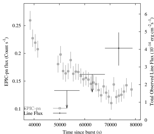
Fig. 4. The light-curve of GRB030227 during the XMM-Newton observation. The continuum (0.2–10 keV) decays steadily during the observations whereas the emission lines become detectable only at the end.
