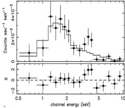
Fig. 6. XMM-Newton EPIC pn spectrum of GRB010220 fitted with a powerlaw and Galactic absorption. The only spectral feature is a possible emission line, which could be due to iron K\alpha , at \sim 3.9 keV (Watson et al. 2002a).
