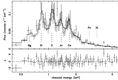
Fig. 3. XMM-Newton EPIC pn spectrum of GRB030227 for the last 11 ksec of the observation (Watson et al. 2003). Top: count-rate spectrum fitted with a powerlaw, Galactic absorption and five Gaussian emission lines. Bottom: chi-squared fit residuals. The identified emission lines are marked at their expected energies for a redshift of z = 1.39 .
