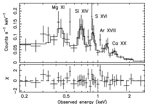
Fig. 1. XMM-Newton EPIC pn spectrum of GRB011211 for the first 5 ksec of the observation (Reeves et al. 2002). Top: count-rate spectrum with best-fit thermal model and Galactic absorption. Bottom: chi-squared fit residuals. The identified emission lines are marked.
