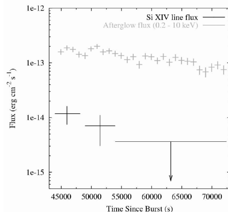
Fig. 2. The decay in the flux of the continuum and the Si XIV line during the XMM-Newton observation of GRB011211. The line is only detected early in the observation.
