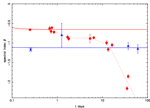
Fig. 8. The observed X-ray (triangles) and optical (circles) spectral indices ( f_\nu \propto \nu^\beta ) as a function of time for GRB030329 (Willingale et al. 2004 and references therein). The dotted line indicates the trend in the optical spectral index. The solid lines show the predicted evolution for the best-fit fireball shock model.
