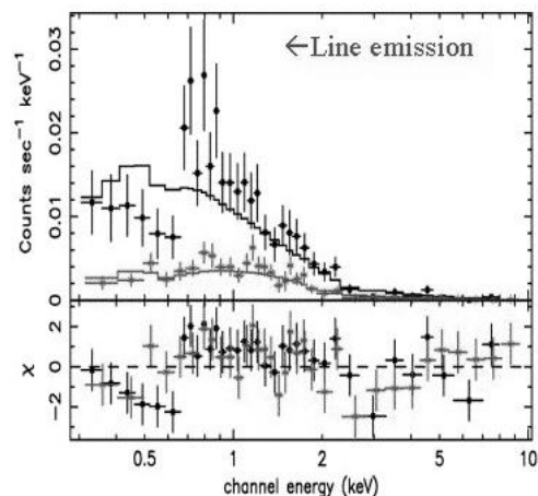
Fig. 5. XMM-Newton EPIC pn and MOS spectra of GRB01025A fitted with a powerlaw and Galactic absorption. There is an excess emission feature observed at \sim 0.8 keV that can be well fitted with a thermal plasma model (Watson et al. 2002a).
