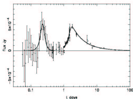
Fig. 9. The residual optical (R band) flux after subtracting the best-fit fireball shock model (Willingale et al. 2004). The curves are simple powerlaw fits for illustration.
