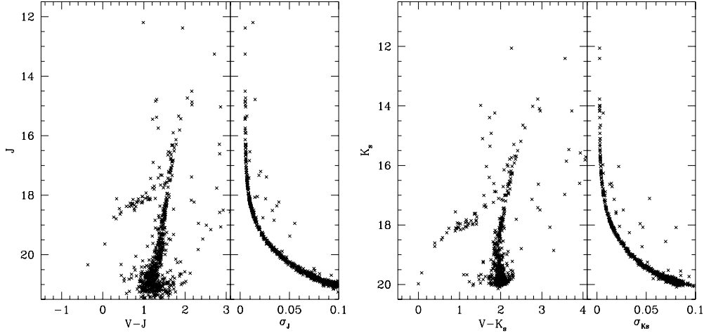
Fig. 1. J-(V-J) (left) and K_s-(V-K_s) color-magnitude diagrams of Reticulum. ALLFRAME mean magnitudes are plotted. We detected \approx 900 stars. The two figures only show stars with DAOPHOT parameters sharpness ( sh ) and \chi (that are diagnostics of the goodness of the photometry) in the range -1 \leq sh \leq 1 and \chi < .6 , respectively.
