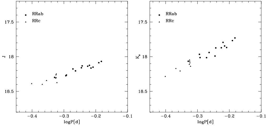
Fig. 2. Observed period-luminosity relations for J (left panel) and K_s -bands. Filled circles depict fundamental pulsators (RRab), while filled triangles are first overtone pulsators (RRc). Periods of RRc have been “fundamentalized” (see text).
