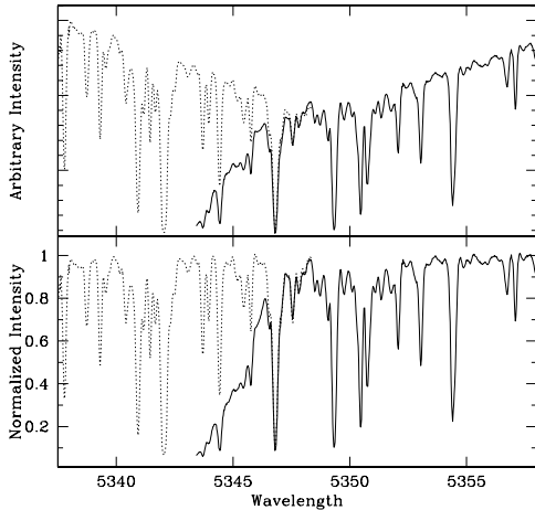
Fig. 1. Example of the automatic normalization procedure applied to the SARG spectrum of HD 44019. Top panel: original data for two adjacent orders, indicated with different line types. Bottom panel: normalized data for the same orders. The procedure works well, except for the extreme blue border of the order more to the red, where the intensity drops too fast.
