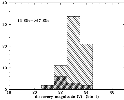
Fig. 2. Magnitude distribution of 13 SNe of the subsample of classified SNe (double shaded histogram) and magnitude distribution of all the candidates (single dashed histogram)
