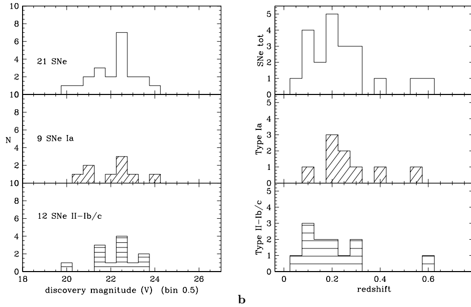
Fig. 1. (a) V magnitude distribution and (b) redshift distribution of the 21 SNe spectroscopically confirmed. Upper panels: type Ia SNe + CCSNe; middle panels: type Ia SNe; lower panels: CCSNe
