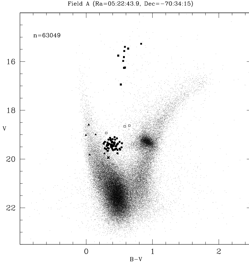
Fig. 1. V vs B - V color - magnitude diagram of Field A from the ALLFRAME reduction of the 2001 data. Different symbols mark the variables identified in this field (RR Lyrae stars: filled circles; anomalous Cepheids: open squares; Cepheids: filled squares; binaries: filled triangles; crosses: \delta Scuti).
