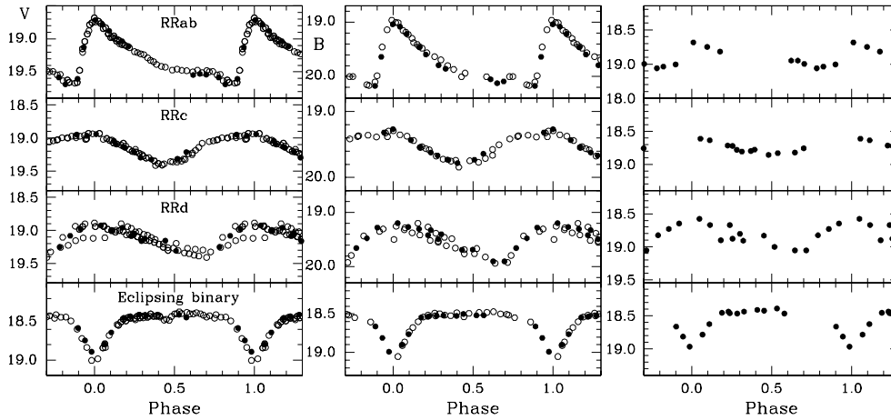
Fig. 2. Some examples of our light curves. Open circles are from Clementini et al. (2001), filled dots are the new data points.
