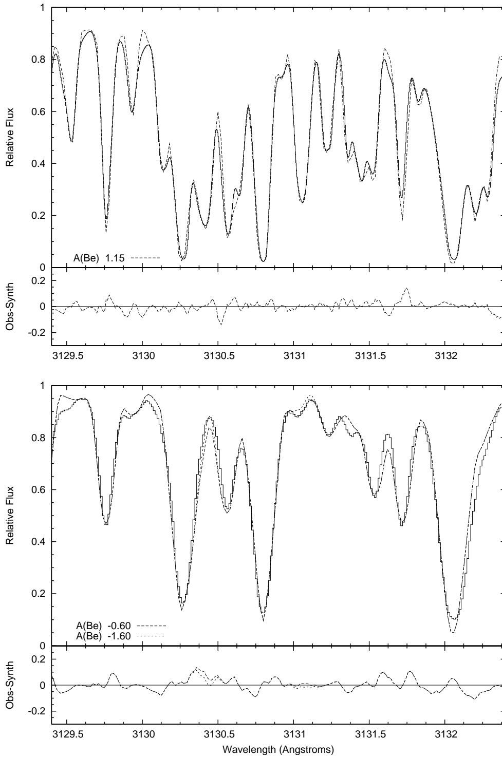
Fig. 1. Spectral synthesis of the Solar Be II doublet (3130.4 Å and 3131.1 Å) region from the NOAO Solar atlas (upper) and Procyon (lower). The upper portion of each plot shows the spectrum (solid line) and synthesis (dashed line). The lower portion of each plot shows the residuals.
