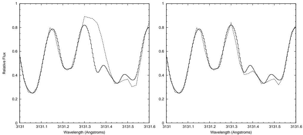
Fig. 3. A magnified section of Figure 1 showing the changes made redward of the Be II doublet. The left plot shows the original Kurucz line list parameters and the right plot shows the fit achieved by adding an OH molecular line (see section 4).
