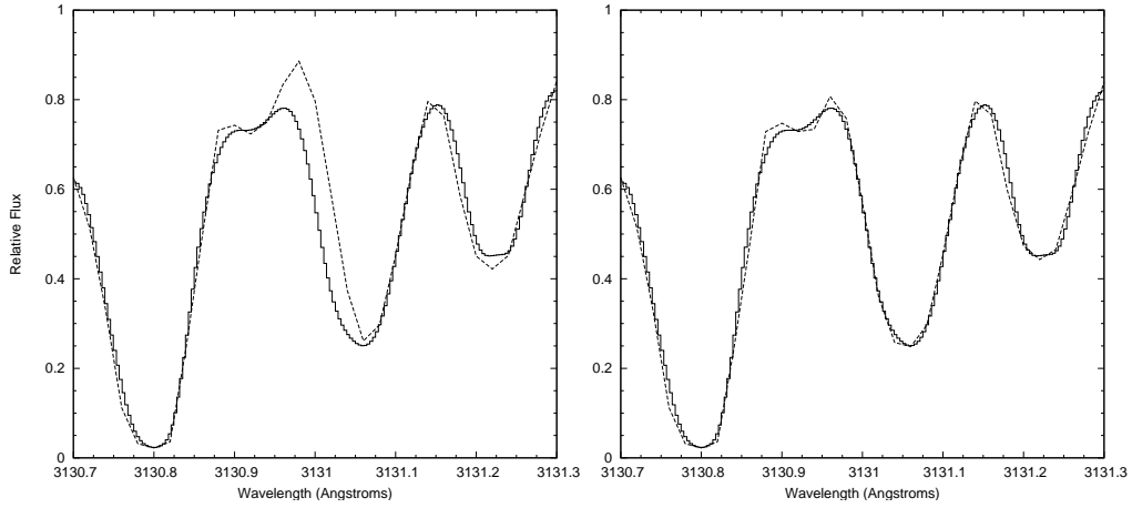
Fig. 2. A magnified section of Figure 1 showing the changes made to the Mn I line at 3131.037 Å. The left plot shows the original Kurucz line list parameters and the right plot shows the fit achieved by altering these parameters (see section 4).
