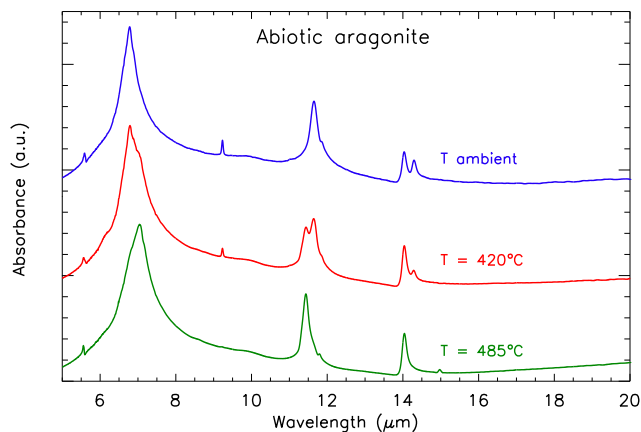
Fig. 1. Abiotic aragonite: before (blue curve) and after thermal process at 420°C (red curve) and at 485°C (green curve). Spectra have been arbitrary scaled for clarity.
