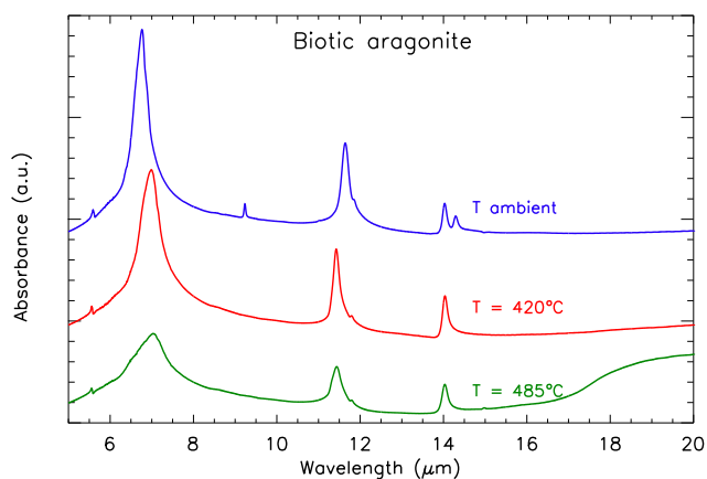
Fig. 2. Biotic aragonite: before (blue curve) and after thermal process at 420°C (red curve) and at 485°C (green curve). Spectra have been arbitrary scaled for clarity.
