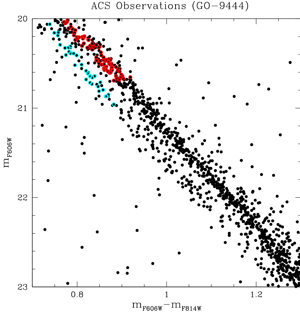
Fig. 1. Color Magnitude Diagram of the \omega Cen Double Main Sequence. In light and dark grey (blue and red in the electronic version) circles are highlighted the targets of the FLAMES+VLT spectroscopic follow-up.
