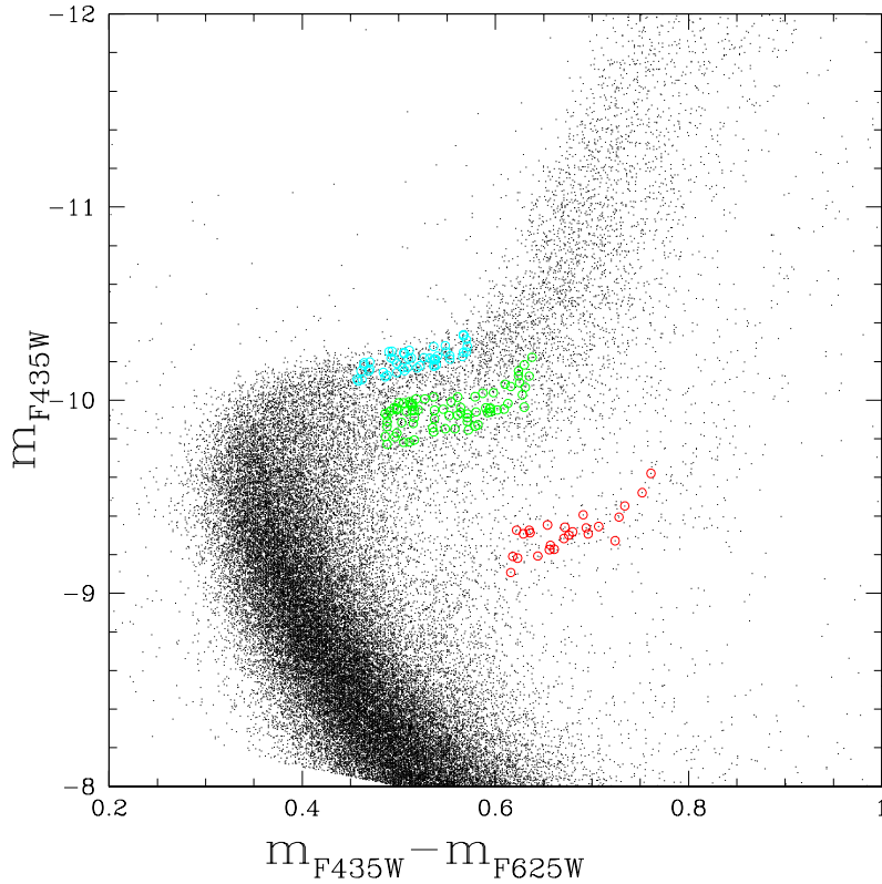
Fig. 2. Instrumental Color Magnitude Diagram around the turn off. Circles highlight the target stars for the spectroscopic follow-up.
