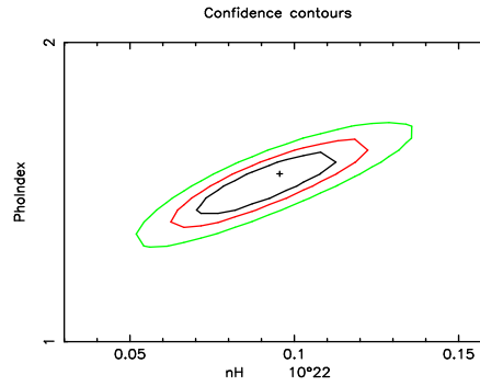
Fig. 4. Confidence contours of the two parameters \Gamma and N_{\text{H}} for the point-source spectrum.
