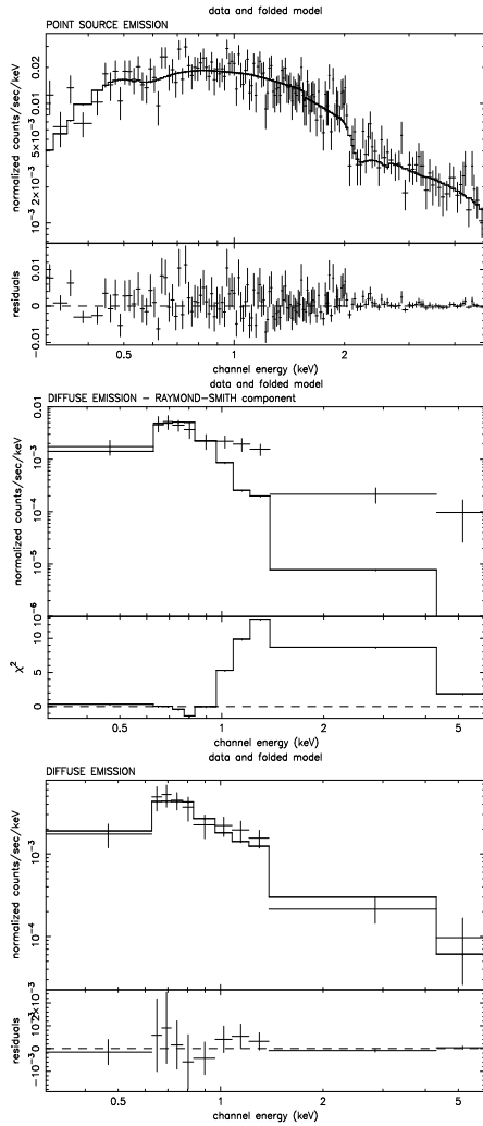
Fig. 3. Top ACIS spectrum of the combined individual unresolved sources. The solid line corresponds to a power law fit with \Gamma = 1.4 and N_{\text{H}} = 9.1 \times 10^{20} \text{ cm}^{-2} . Center ACIS spectrum of the diffuse component: even if the statistics is low, the spectrum can not be fitted by a single component. We show here the fit with a hot plasma component only: the hard tail is evident. The same kind of residuals is obtained by the fit with a power law component only. Bottom The same ACIS spectrum for the diffuse component: we show here the fit with a hot plasma component plus power law (see text for details).
