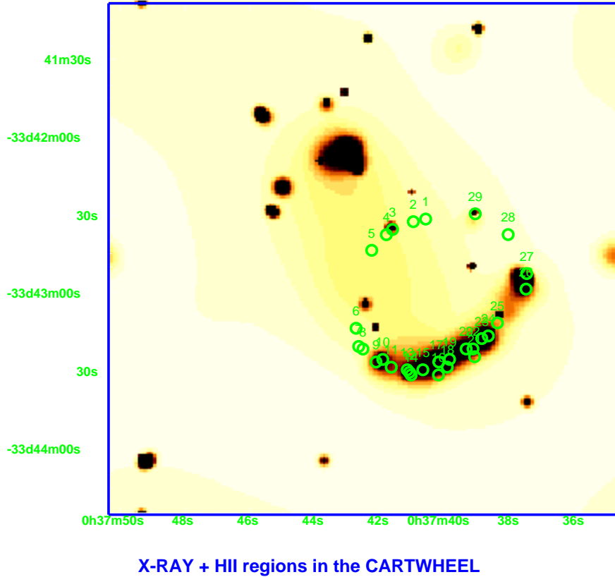
Fig. 2. The ACIS-S image, smoothed with csmooth . The circles mark the position of the HII knots measured by Higdon (1995).
