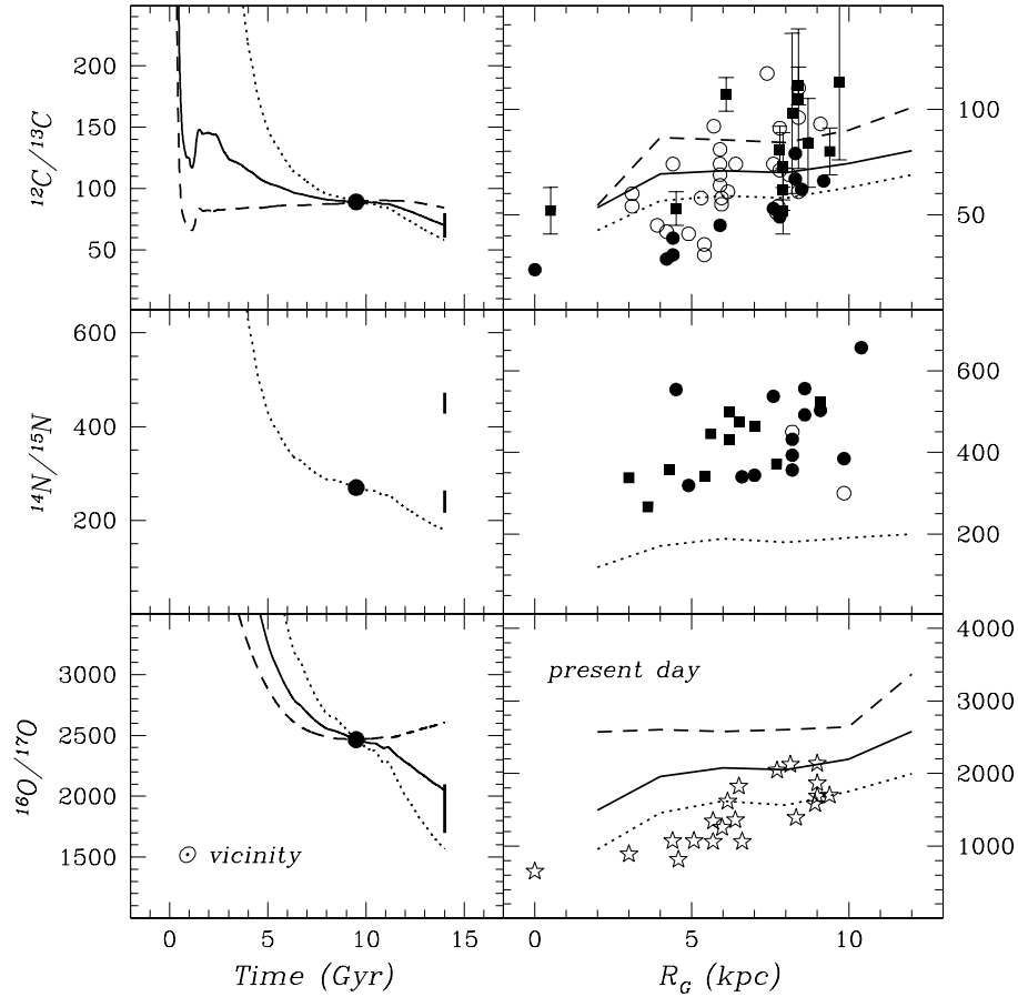
Fig. 2. Theoretical evolution of ^{12}\text{C}/^{13}\text{C} (upper panels), ^{14}\text{N}/^{15}\text{N} (middle panels) and ^{16}\text{O}/^{17}\text{O} (lower panels) in the solar vicinity (left panels) and across the Galactic disc at the present time (right panels), versus observations. See text for details.
