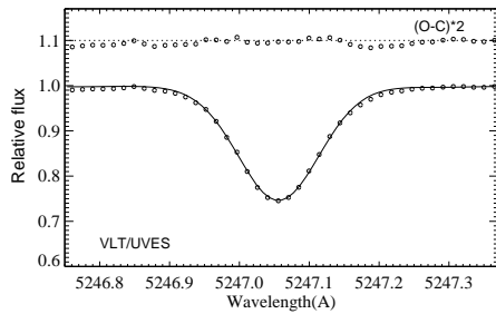
Fig. 1. The best fit (continuous curve) of the Fe I 5247 Å line in HD 122563 (open circles) obtained from the NLTE calculations with the MAFAGS-OS model 4600/1.60/−2.5. The theoretical profile was convolved with a profile that combines instrumental broadening with a Gaussian profile of 3 \text{ km s}^{-1} and broadening by macroturbulence with a radial-tangential profile of 4 \text{ km s}^{-1} . The differences between observed and calculated spectra (O - C) multiplied by a factor of 2 are presented in the upper part of figure (offset by +1.1).
