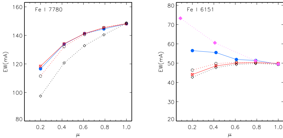
Fig. 3. Solar observed (filled circles) and predicted centre-to-limb variations of line equivalent widths for Fe I 7780 Å (left panel) and Fe I 6151 Å (right panel). Filled rombs (only for Fe I 6151 Å) correspond to full 3D-LTE line formation, crossed open circles to the NLTE calculations with the \langle 3D \rangle model, open circles to LTE with \langle 3D \rangle , and open rombs to LTE with the MAFAGS-OS model.
