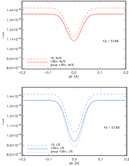
Fig. 4. Theoretical NLTE (top panel) and LTE (bottom panel) fluxes (in \text{erg cm}^{-2} \text{s}^{-1} \text{Hz}^{-1} ) for Fe I 5166 Å from the \langle 3D \rangle_{12} (group \langle 3D \rangle , dotted curve), \langle 3D \rangle (continuous curve), and 1D_{\text{LHD}} (dashed curve) models 4480/2/-3. All the computations were performed with \log gf = -5.2 and \xi_i = 1.8 \text{ km s}^{-1} .
