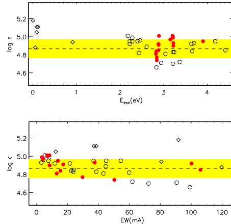
Fig. 2. NLTE ( S_{\text{H}} = 0.1 ) abundances derived from the Fe I (open circles for E_{\text{exc}} \geq 2 \text{ eV} and rombs for E_{\text{exc}} < 2 \text{ eV} ) and Fe II (filled circles) lines in HD 122563 as a function of excitation energy of the lower level (top panel) and observed equivalent width (bottom panel). In each panel, the dashed line shows the mean iron abundance determined from the Fe I E_{\text{exc}} \geq 2 \text{ eV} lines.
